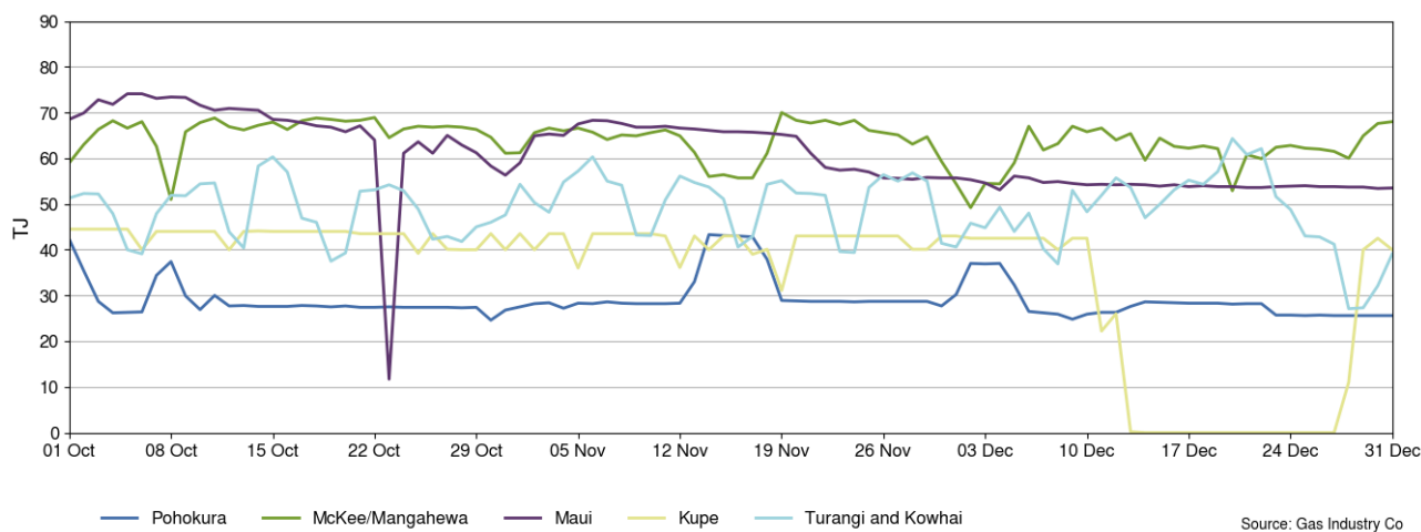
Figure 13: New Zealand gas production, October to December 2024
