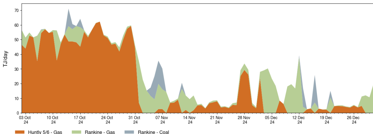
Figure 15: Estimated Huntly fuel consumption, October–December 2024
